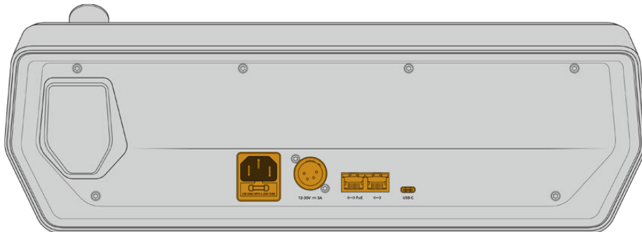
ATEM 1 M/E Advanced Panel后面板的各个接口
