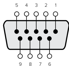
RS-422 PTZ-Pinbelegung
