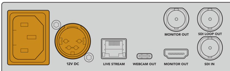
Blackmagic Web Presenter can be powered using the IEC or 12V DC power input
